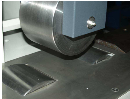
Precise leveling by two right-left movable bottom pressure rollers, one idle top, up-down movable roller.
