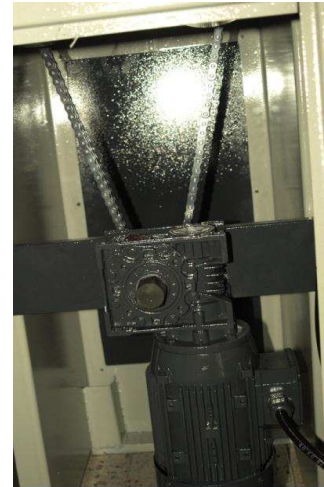
Movement transmission to pressure rollers by motor driven chain.
